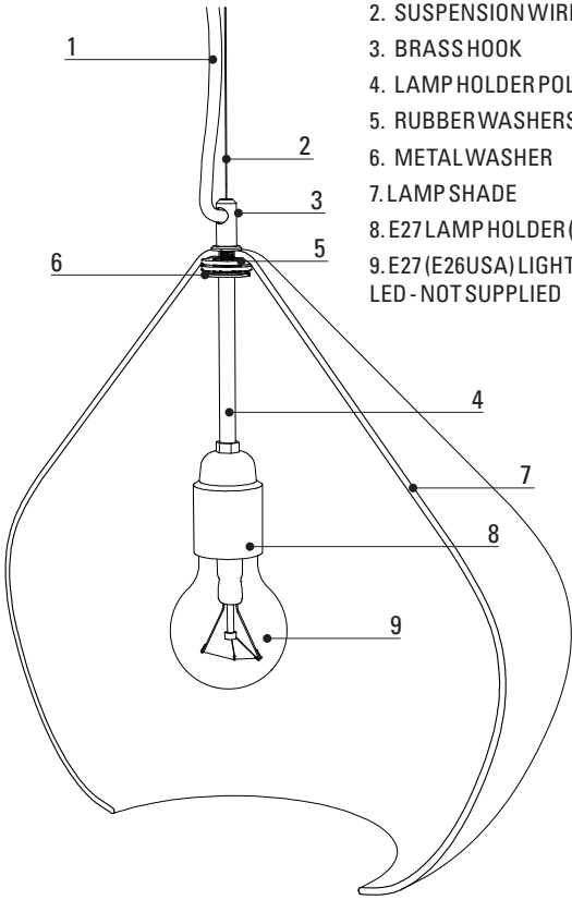
DIAGRAM 1 Lamp Components
