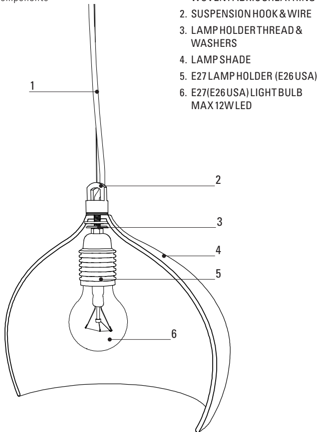
DIAGRAM 1 Lamp Components
